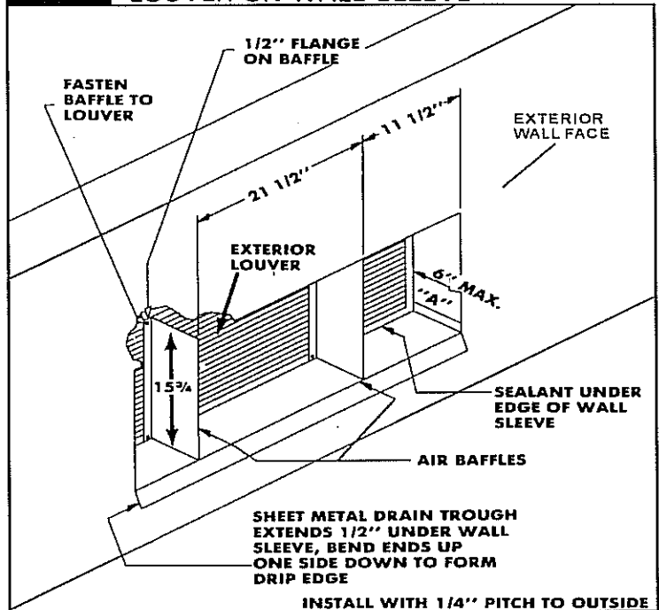
FIG. 4 DEEP WALL WITH STAMPED LOUVER ON WALL SLEEVE
